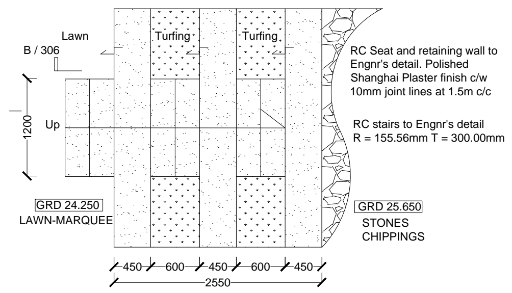
A 101 PLAN : Pool Deck Terraces down to Lawn-Marquee 1: 50
