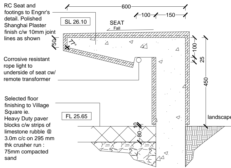
D 306 DETAIL : VILLAGE SQUARE RC Seating - Section 1: 50
