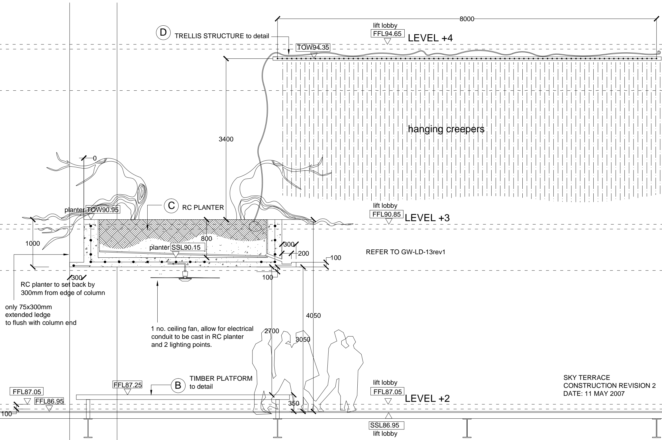
SECTION Y : Typical Sky Terrace (Level +2, +6, +10, +13, +16, +19) scale 1:50
