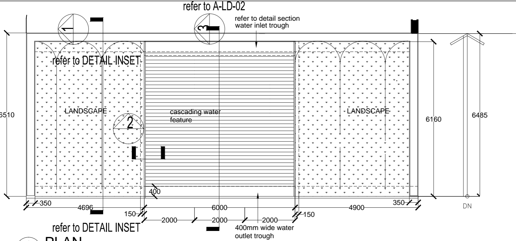
A PLAN Scale 1:100
