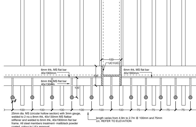
DETAIL PLAN C scale 1: 5
