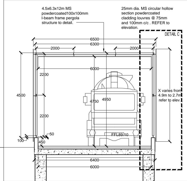
SECTION B scale 1: 50
