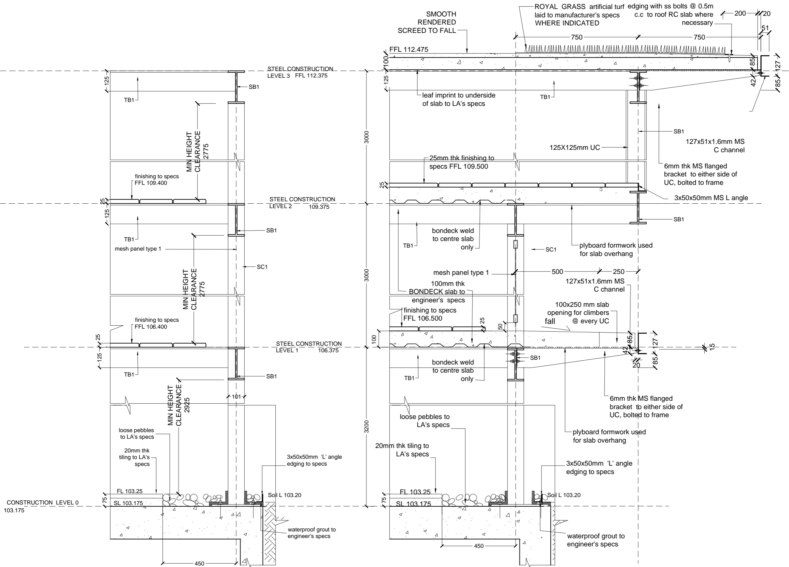
TYPICAL SECTION: CONSERVATORY FRAME scale 1:15
