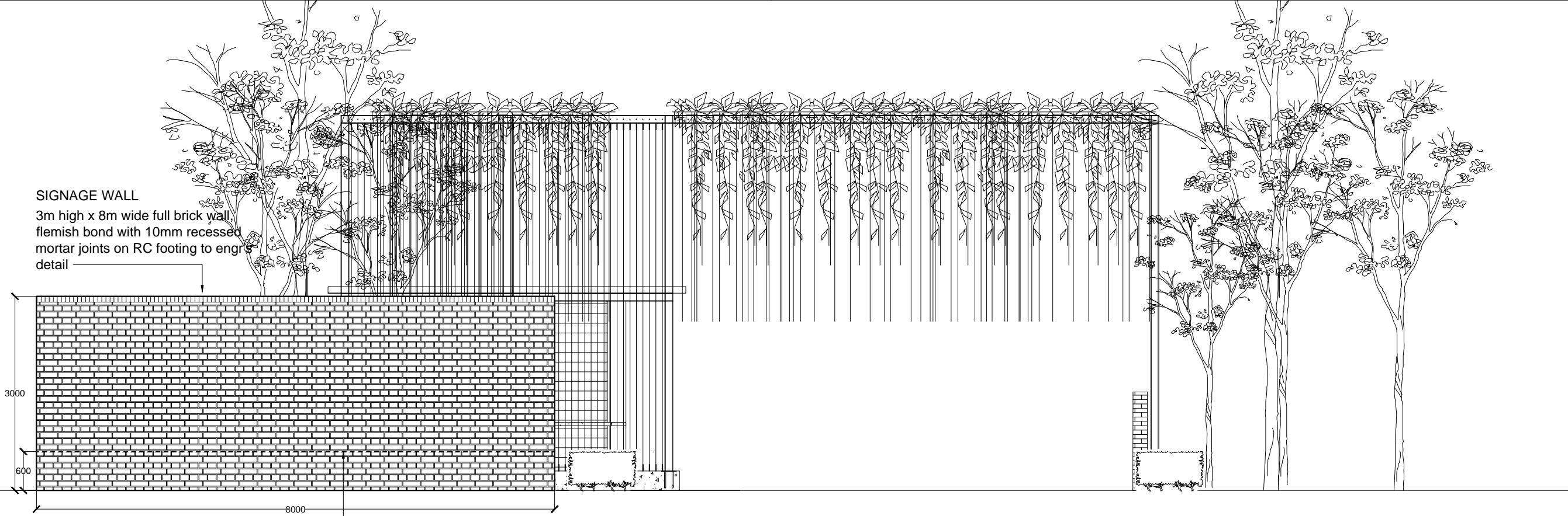
BRICK SIGNAGE WALL Scale 1:75
