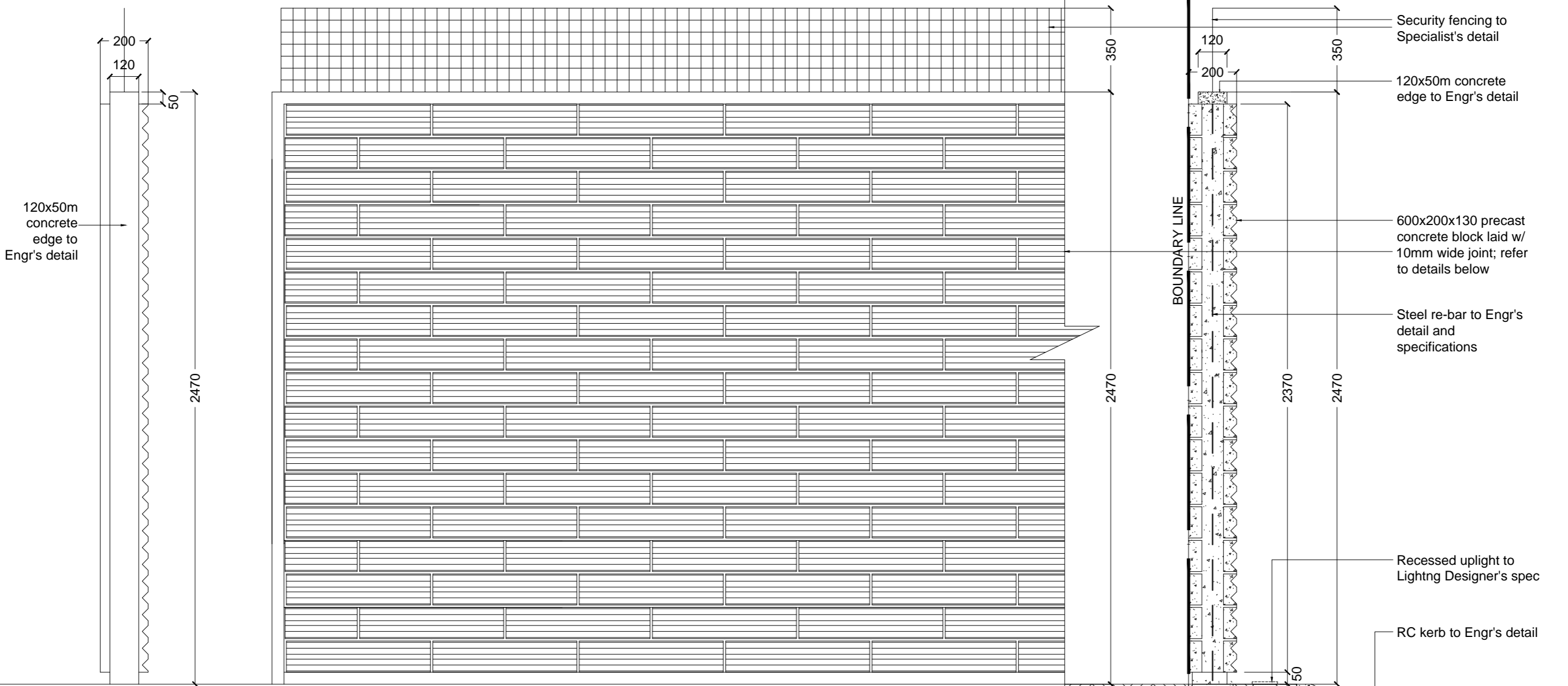
SIDE ELEVATION: FEATURE WALL SCALE 1:20
