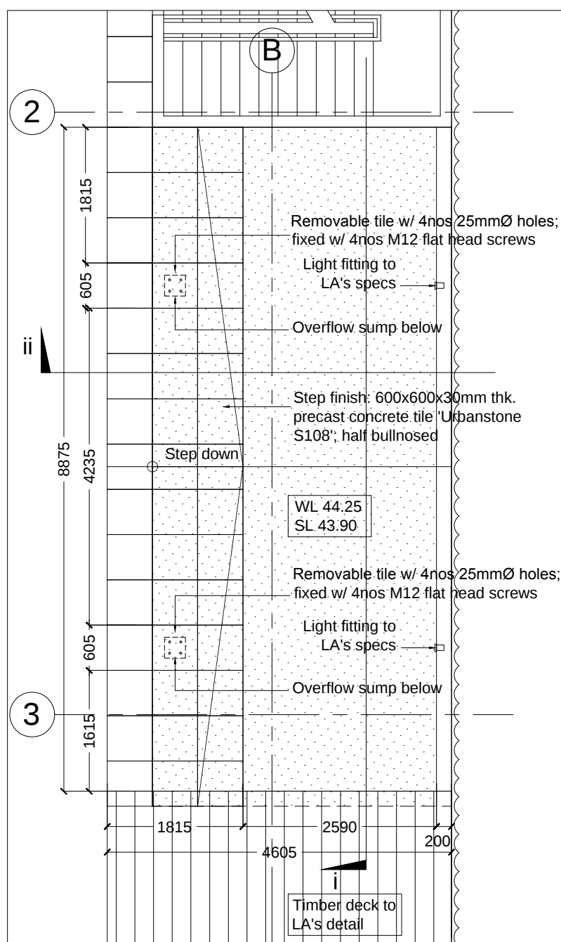
PLAN : CHILDREN'S POOL SCALE 1:75
